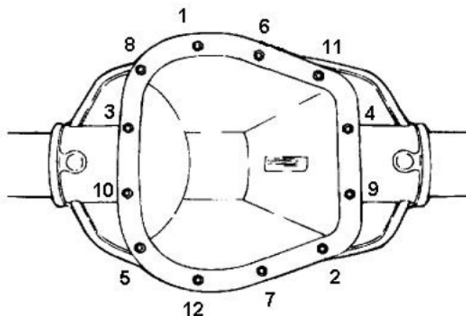
Figure 2: Cross Tight Pattern and Torque Specifications
